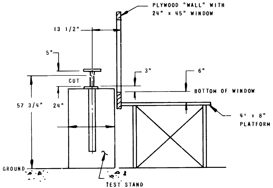
Figure 5-7. Mockup of Physical Constraints at RV Head
