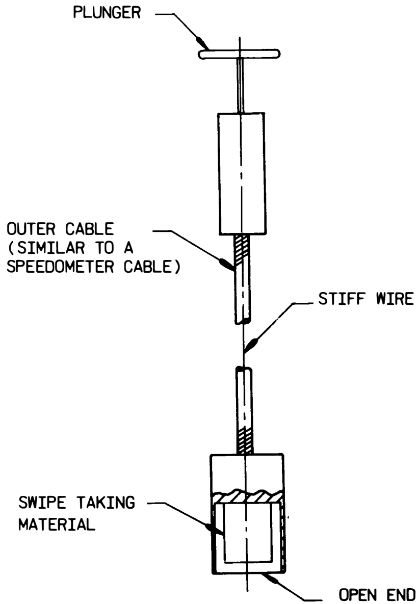
Figure 3-22. Swipe Sampler
