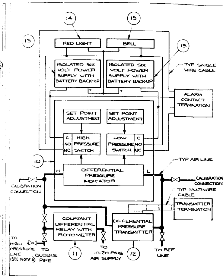
BLOCK DIAGRAM SEE NOTE 1 SCALE: NONE
