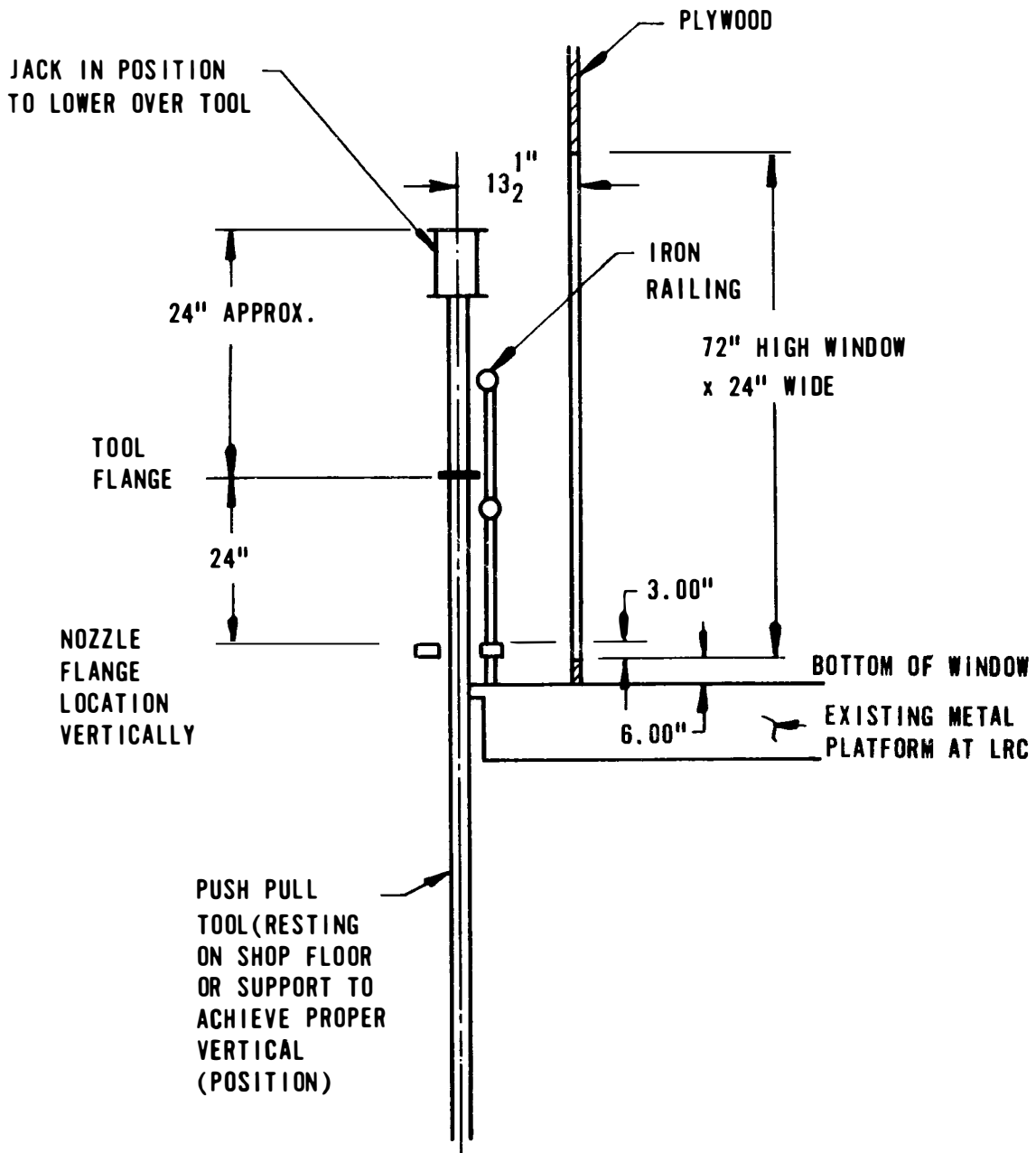
Figure 5-11. Push-Pull Mockup at LRC (B&W Lynchburg)
