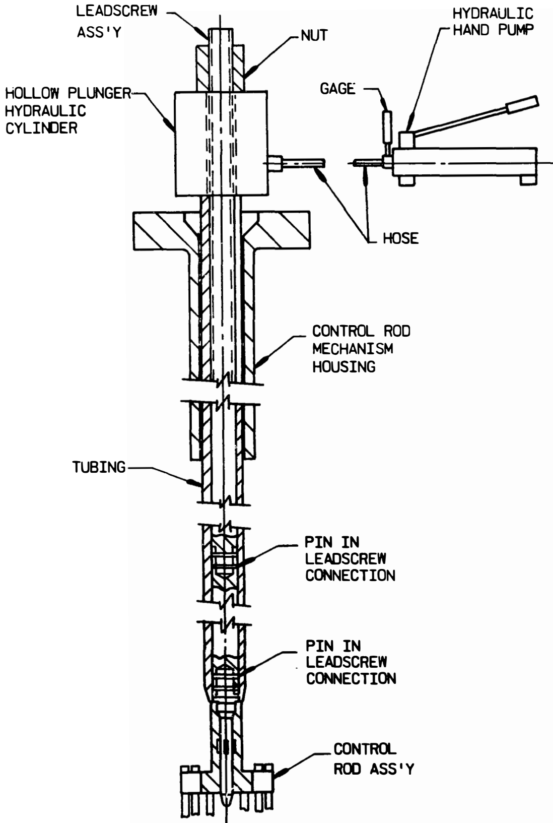
Figure 3-16. Leadscrew Puller/Separator
