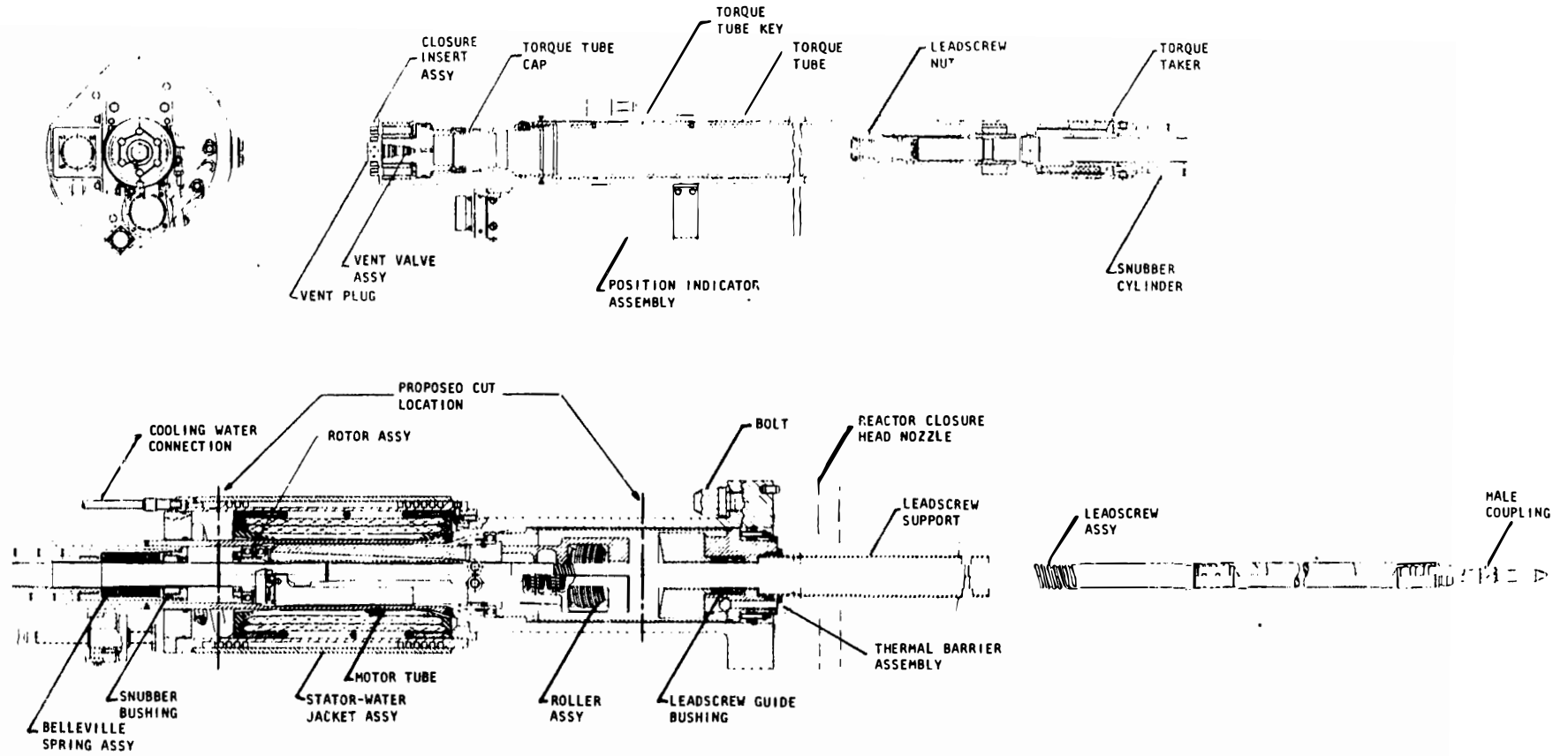
Figure 3-12. Control Rod Drive Mechanism
