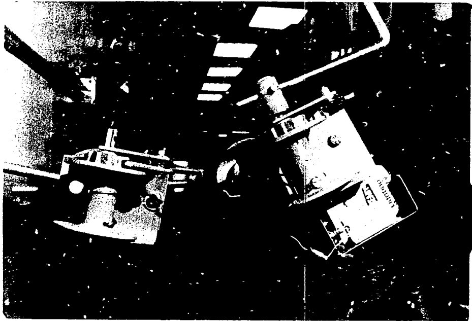
Figure 4-28. In-Head Leadscrew Cutting Tools
