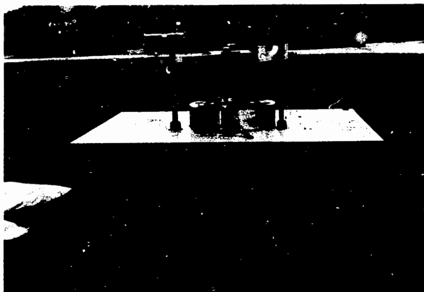
Figure 5-9. Mockup of Ex-Head Leadscrew Plasma-Arc Cutting
