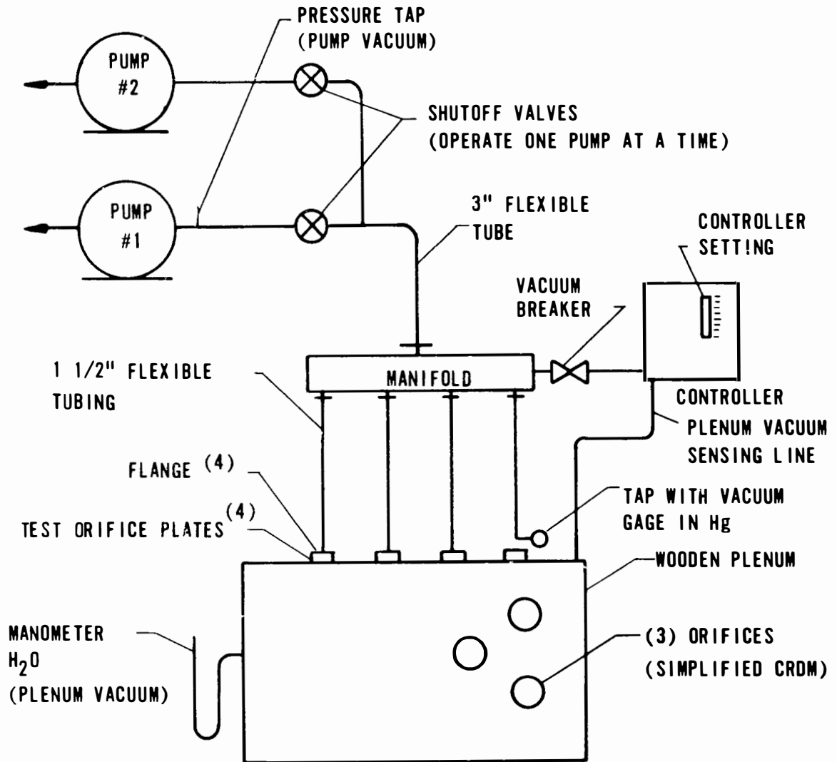
Figure 5-12. Purge System Mockup at B&W Special Products
