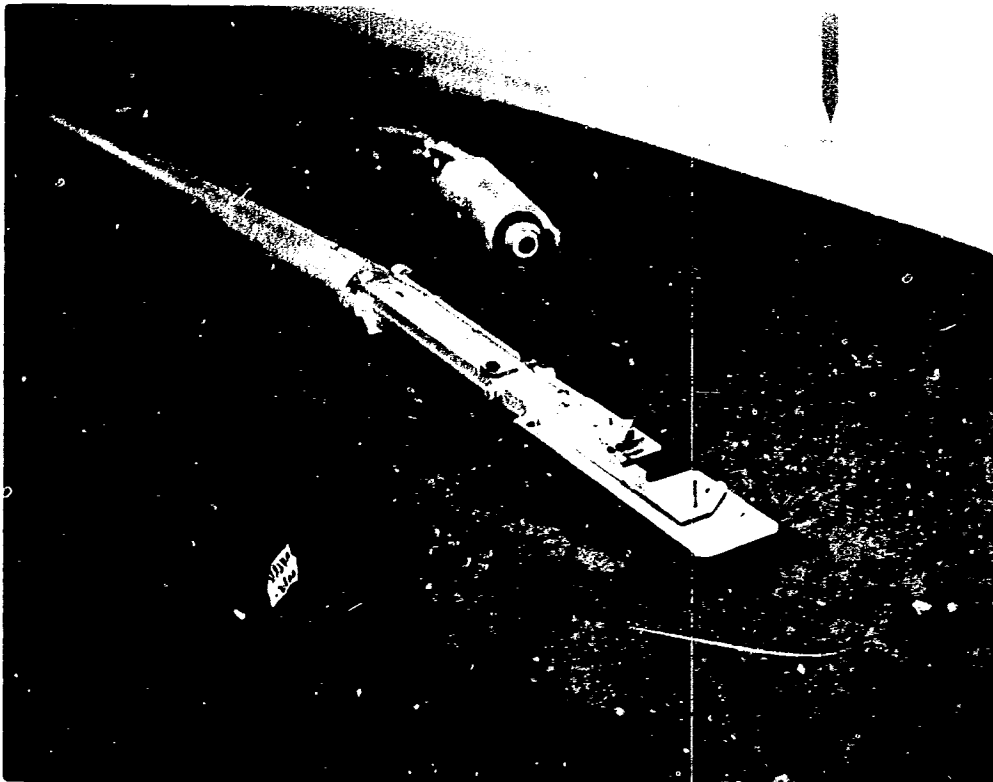
Figure 4-26. Underhead Plasma Cutter and Clamp
