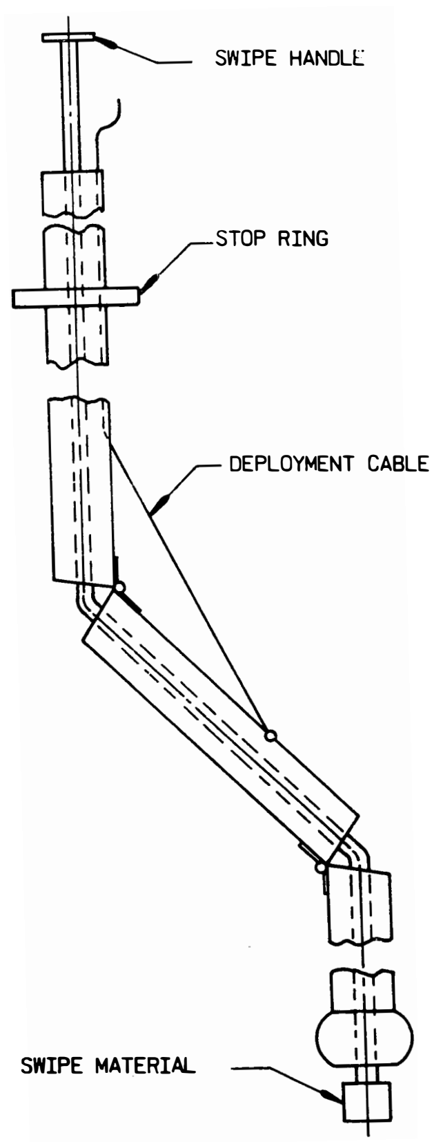
Figure 3-21. Manipulator for Swipe Sampling
