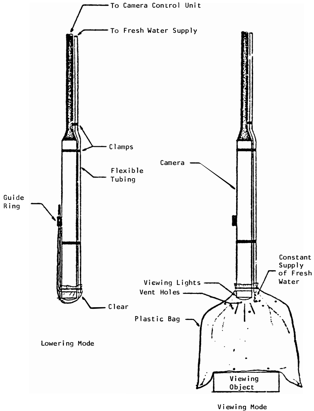
Figure 3-18. Concept for Murky Water Viewing
