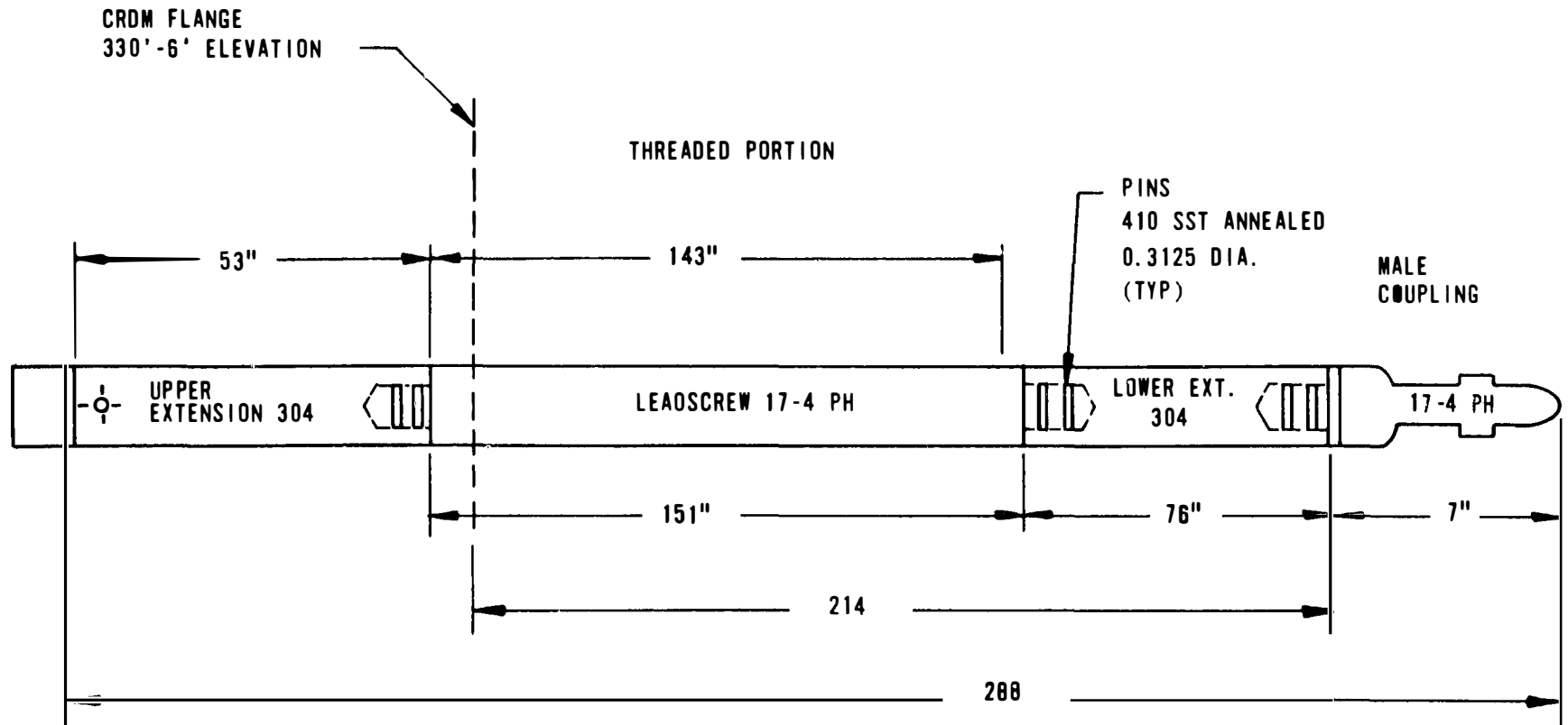
Figure 3-13. Leadscrew Assembly
