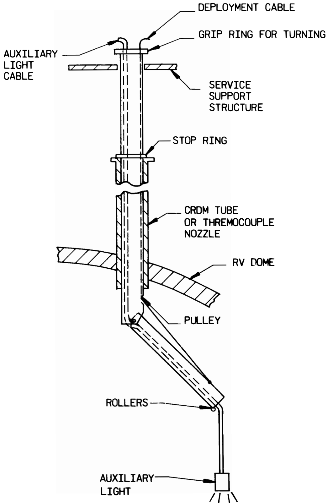
Figure 3-20. Hinged Tube Manipulator for Auxiliary Lights
