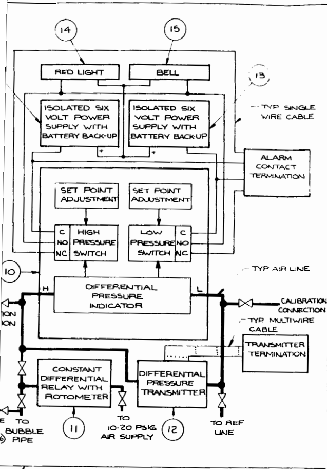
5 BLOCK DIAGRAM SEE NOTE 1 SCALE: NONE
