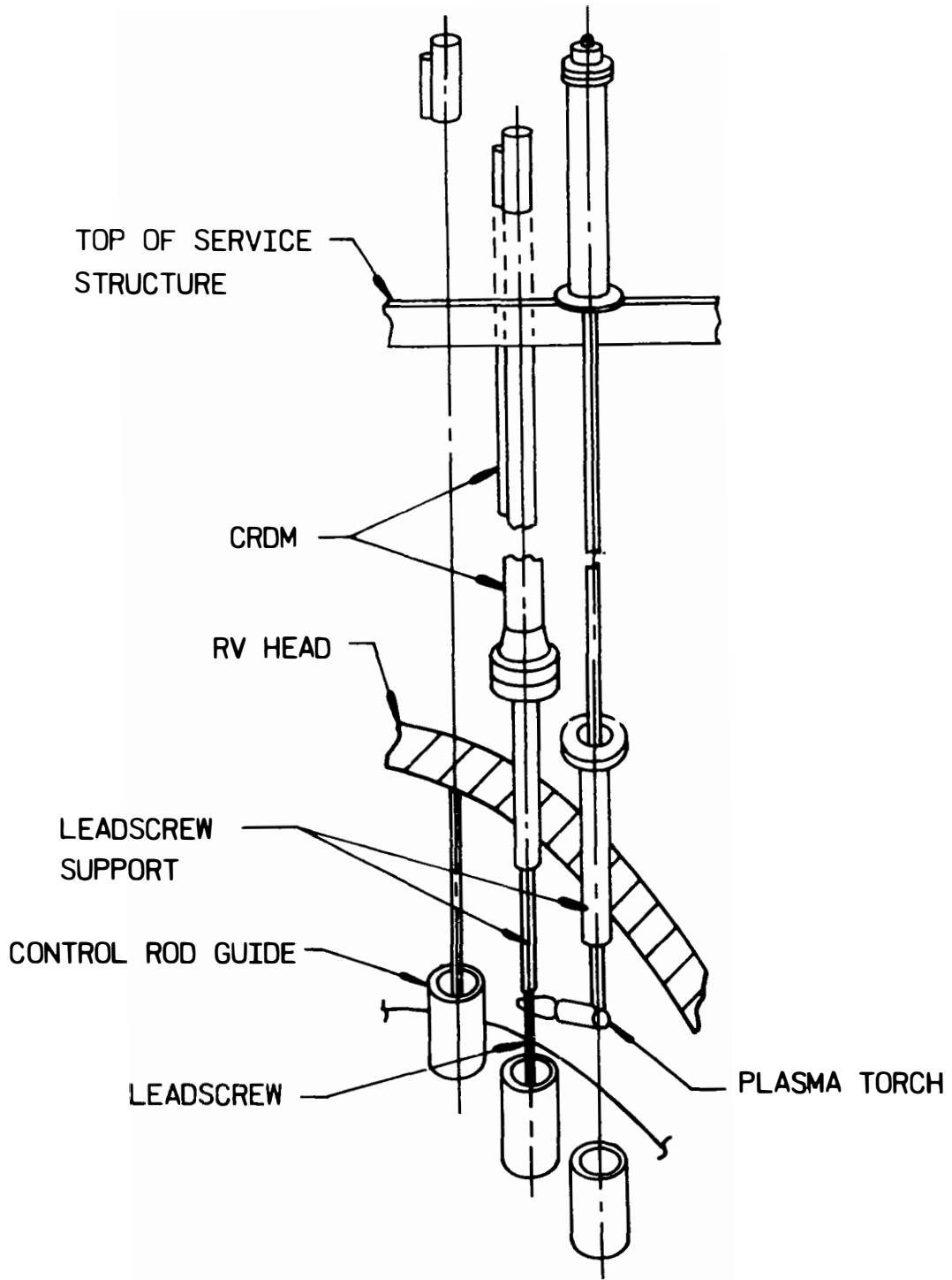
Figure 3-17. In-Head Leadscrew Cutter
