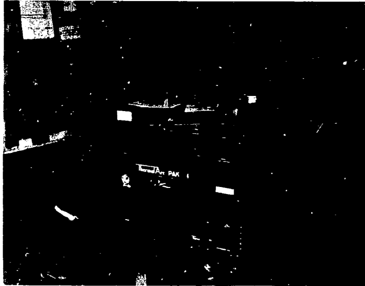
Figure 5-8. Mockup of Ex-Head Leadscrew Plasma-Arc Cutting
