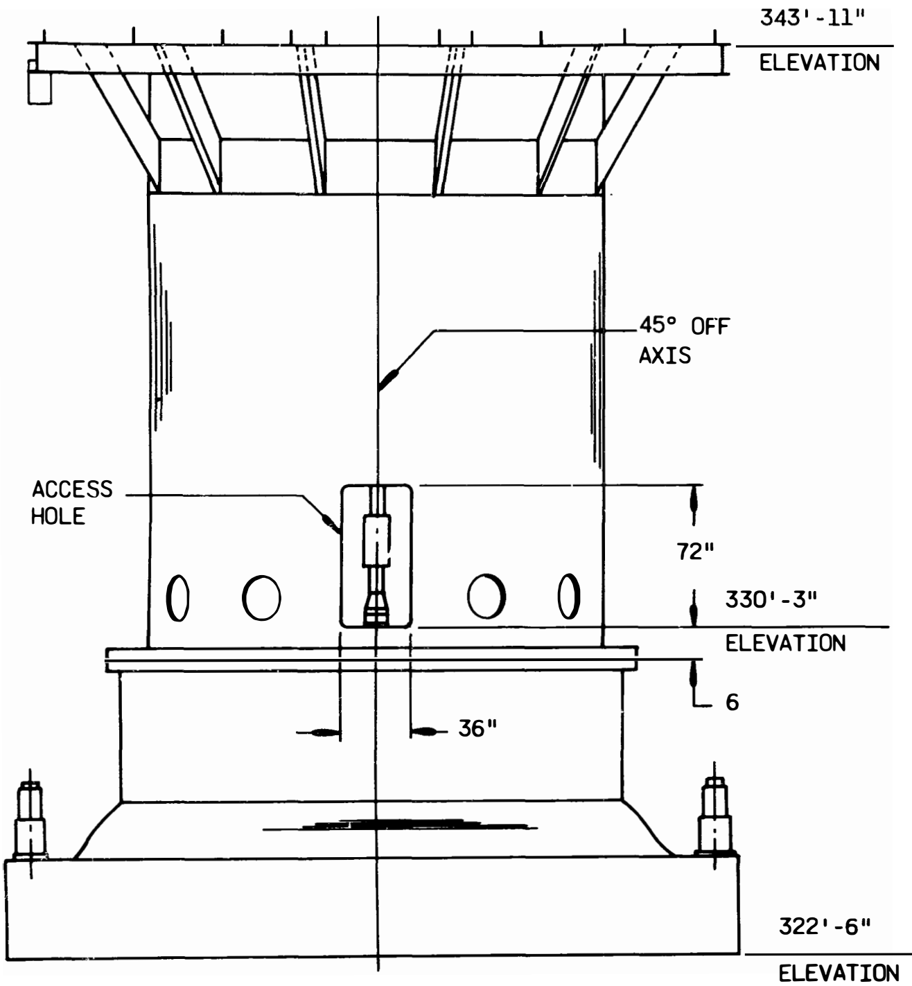
Figure 3-11. CRDM Access Hole in Service Structure
