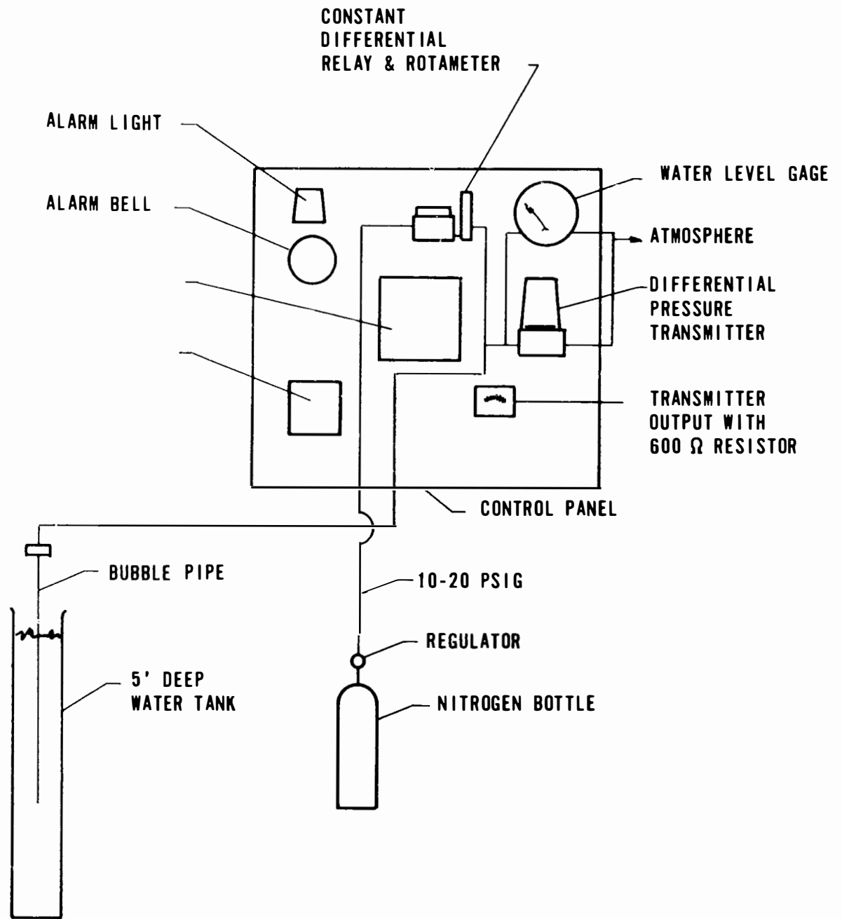
Figure 5-13. Water Level Mockup at B&W Special Products
