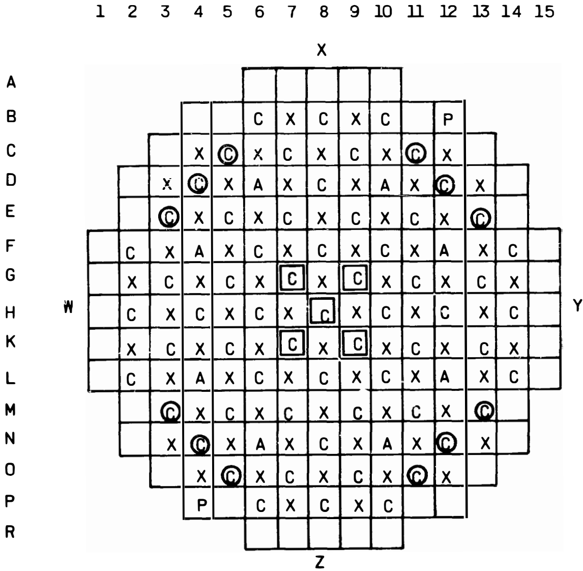
Figure 2-1. Location of Control Assemblies
