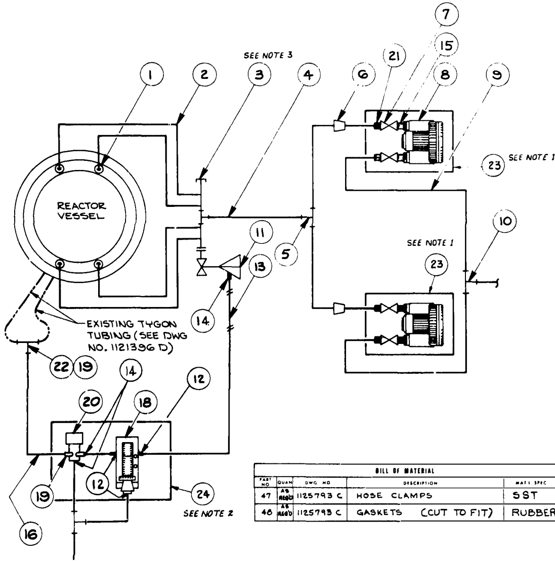
Figure 4-1. Purge System
