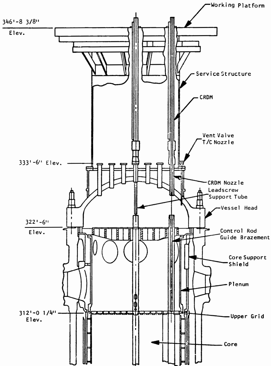
Figure 4-25. Reactor and Service Structure
