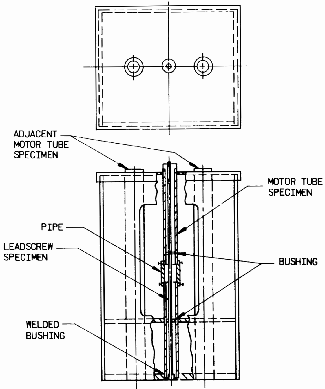
Figure 3-24. Motor Tube/Leadscrew Cutting Mockup
