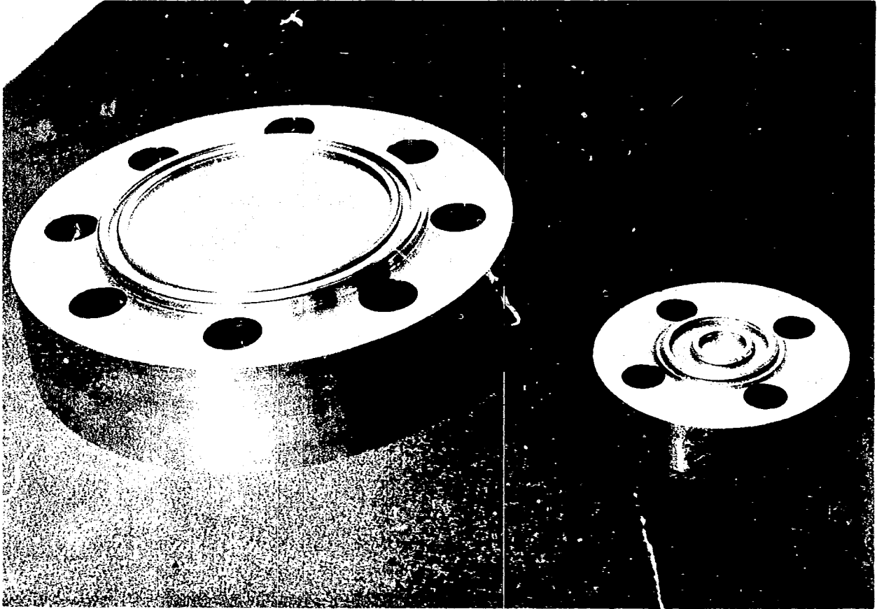
Figure 4-11. CRDM and Thermocouple Nozzle Blind Flanges
