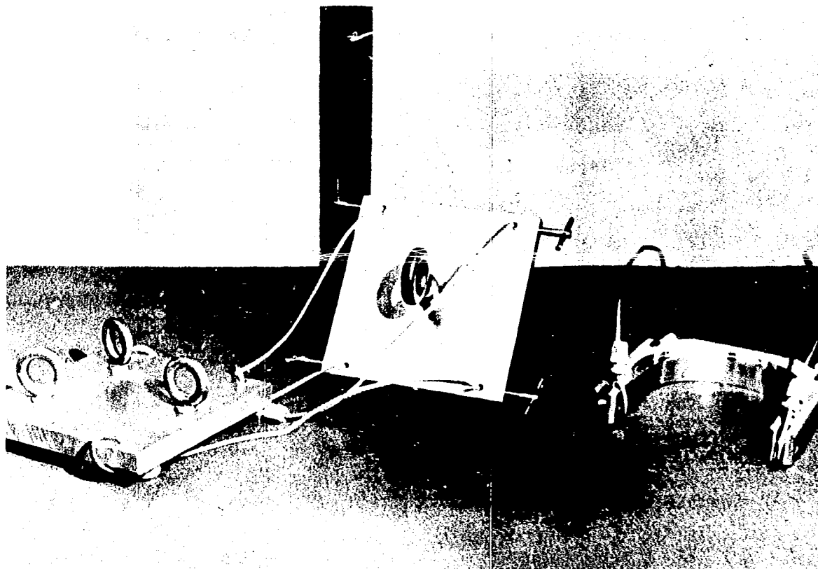
Figure 4-18. Stator Removal Tool
