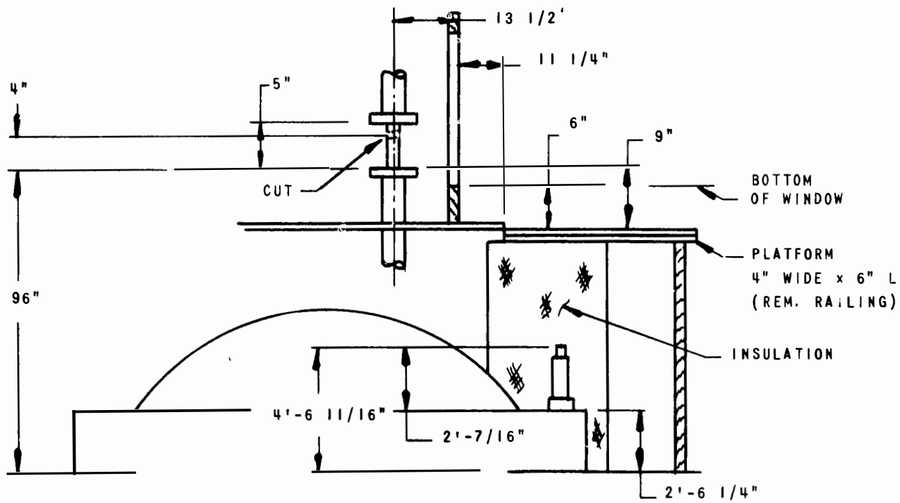
Figure 5-6. Location of Platform for Ex-Head Cutting
