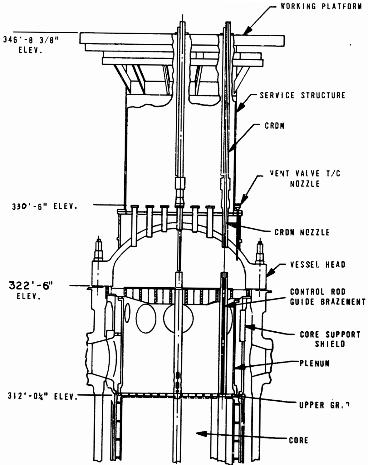
Figure 2-2. Reactor and Service Structure
