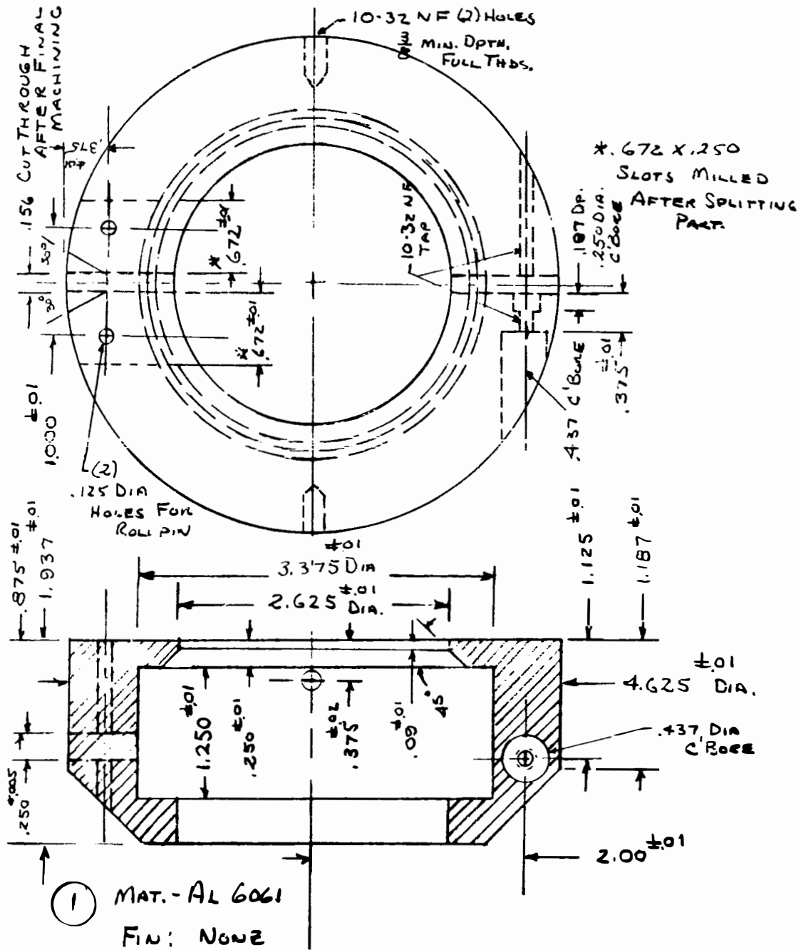
Figure 4-20. Leadscrew Support Tube Clamp
