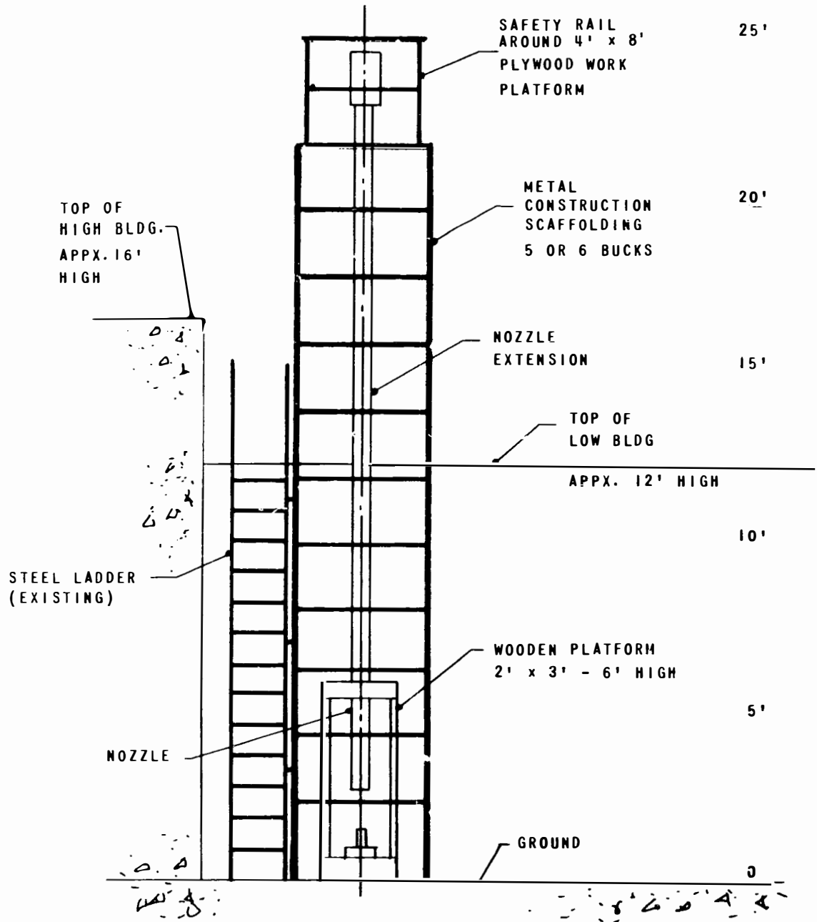
Figure 5-10. Mockup In-Head Cutting
