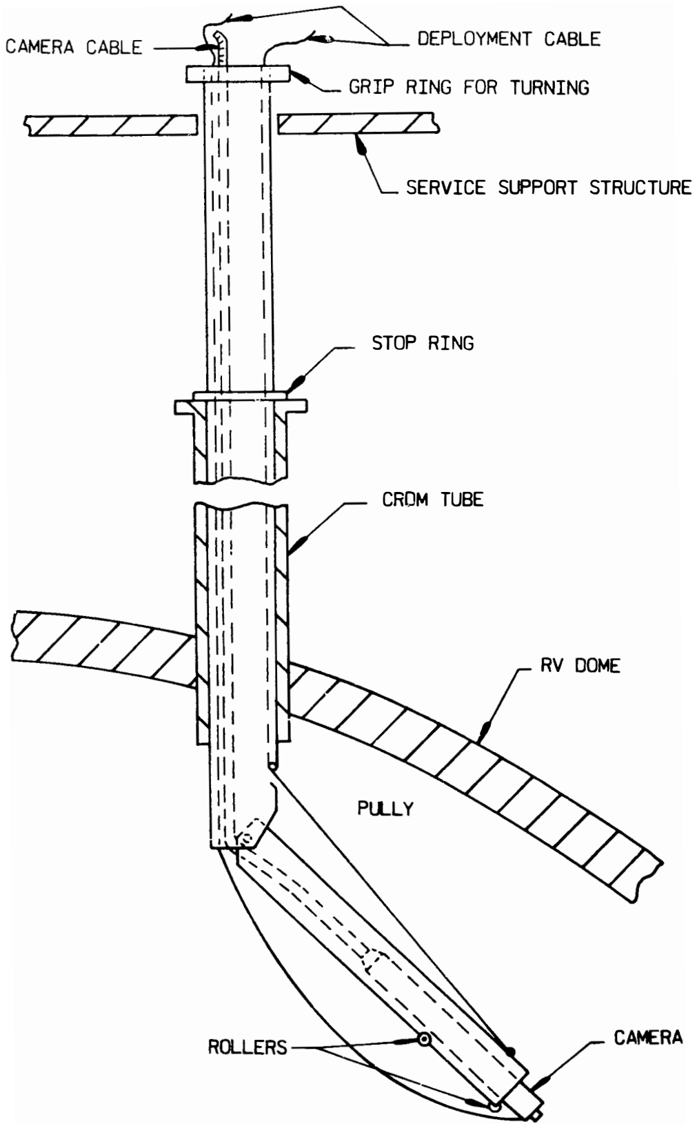
Figure 3-19. Option Using CRDM Tube From SSS
